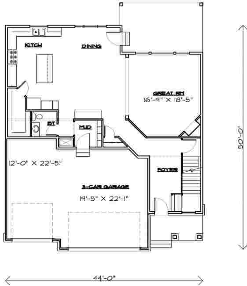
Main floor
