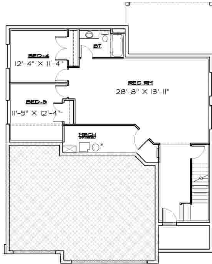
Basement
